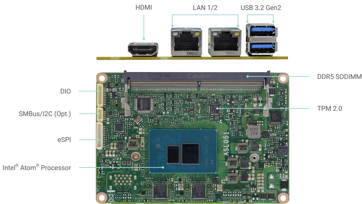
Bottom View
