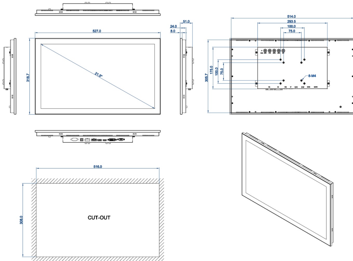
DIMENSIONAL DRAWING:TM-PCA215
