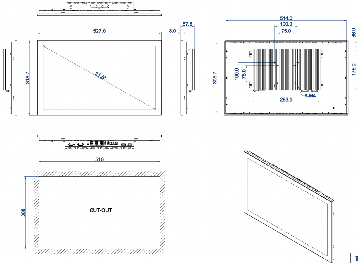
DIMENSIONAL DRAWING:TPC-DCS215E/T
