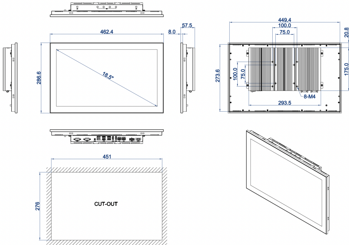
DIMENSIONAL DRAWING:TPC-DCS185E/T
