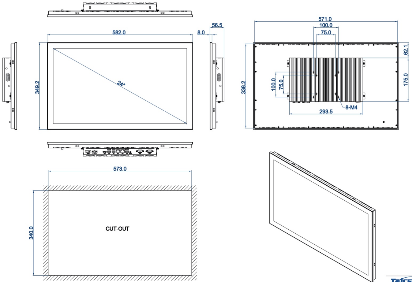
DIMENSIONAL DRAWING:TPC-DCM240W
